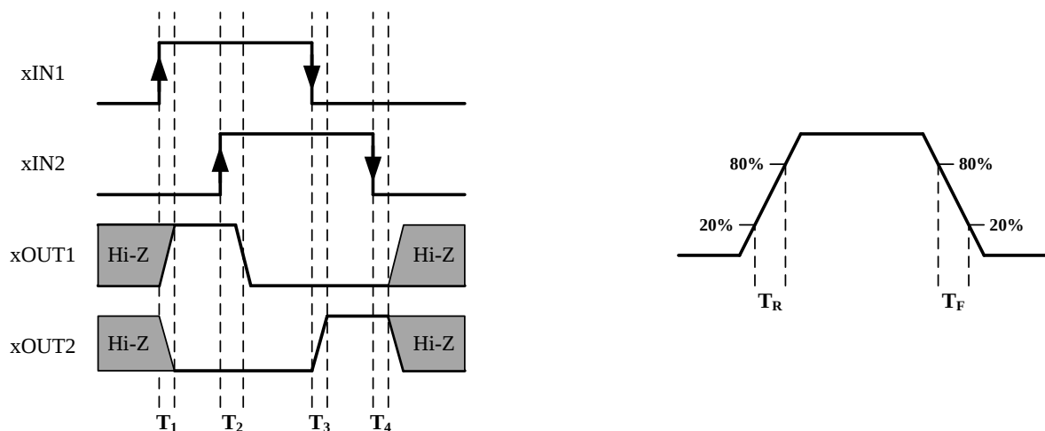
Figure 6-1. Timing Diagram
