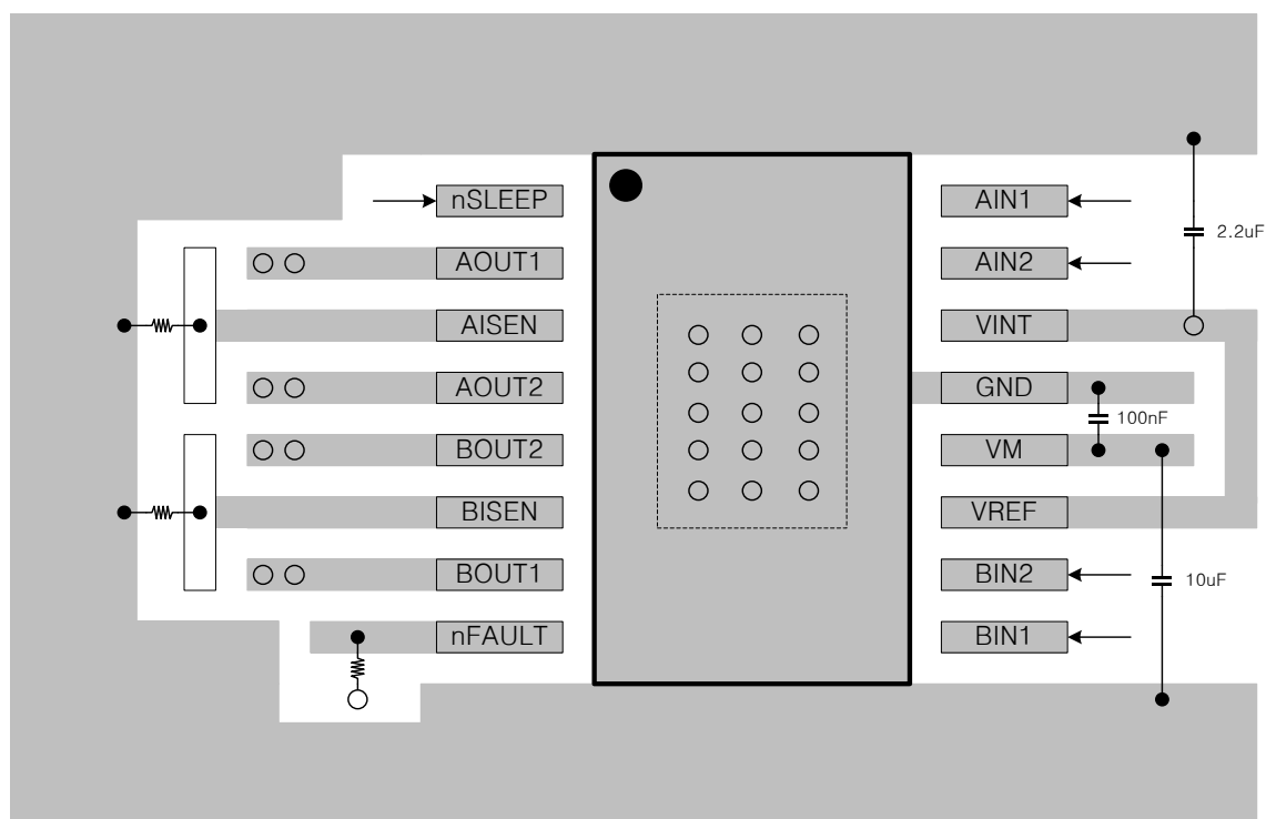
Figure 10-1. Layout Recommendation
