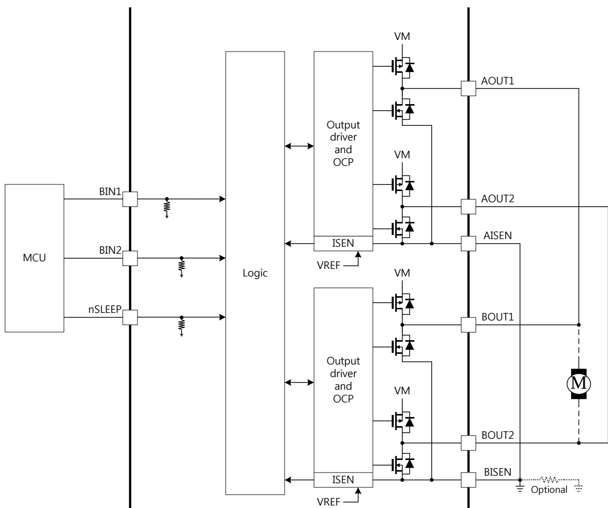
Figure 7-2. Parallel Mode Operation
